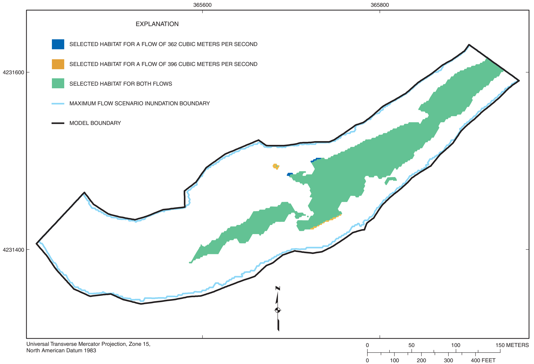
Figure 4-37. Selected habitat area distribution for habitat category 7 (paddlefish) at flows of 362 and 396 cubic meters per second at Marais des Cygnes River site MDC2.
